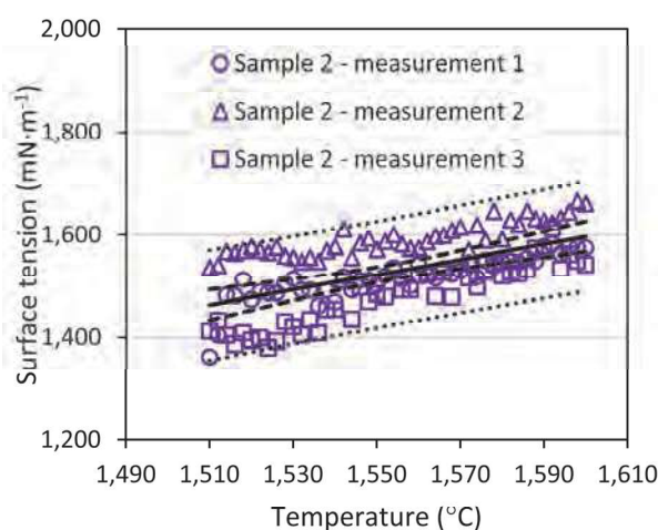
Fig. 3 Temperature dependencies of the surface tension for the sample 2 (1.925 wt. % Cr)
