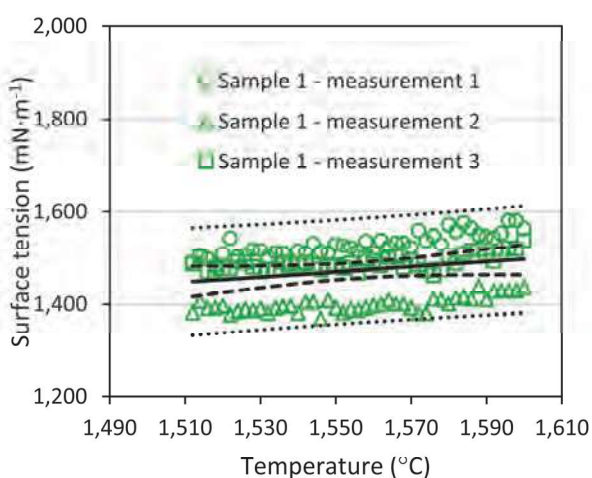
Fig. 2 Temperature dependencies of the surface tension for the sample 1 (0.924 wt. % Cr)
