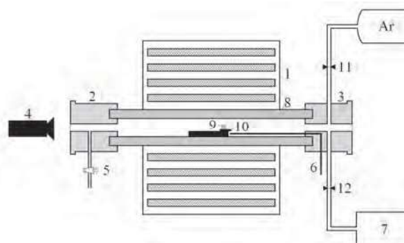
Fig. 1 Schematic illustration of the observation furnace Clasic 1) heating elements, 2) front flange, 3) rear flange, 4) CCD camera, 5) high-vacuum stopcock, 6) type B thermocouple, 7) vacuum pump, 8) alumina tube, 9) sample, 10) alumina substrate, 11) gas inlet, 12) gas outlet
