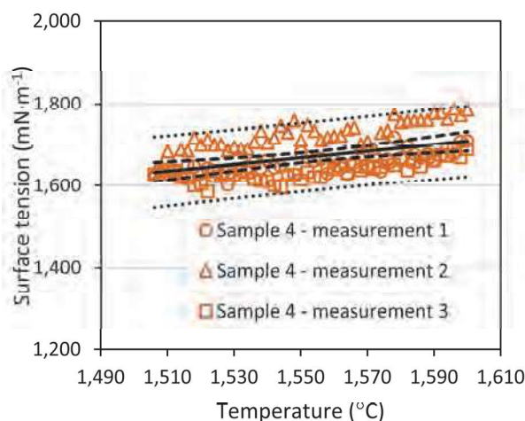
Fig. 5 Temperature dependencies of the surface tension for the sample 4 (3.772 wt. % Cr)
