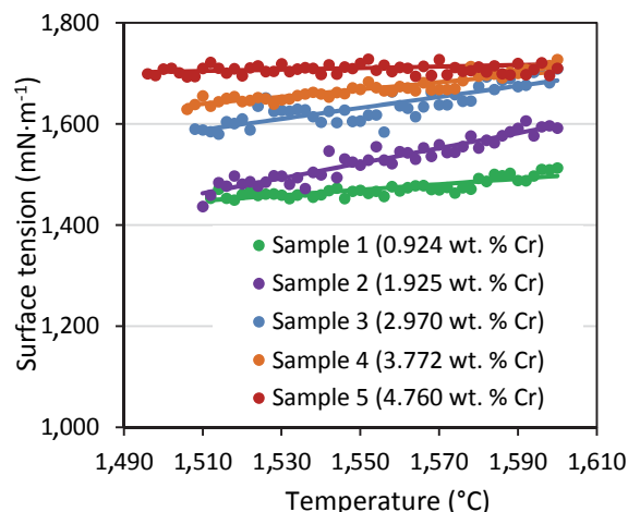
Fig. 7 Dependencies of average surface tension on the temperature for the samples 1 – 5
