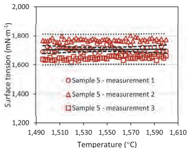
Fig. 6 Temperature dependencies of the surface tension for the sample 5 (4.760 wt. % Cr)
