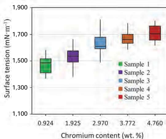
Fig. 8 Boxplot of chromium effect on the surface tension
