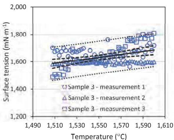
Fig. 4 Temperature dependencies of the surface tension for the sample 3 (2.970 wt. % Cr)
