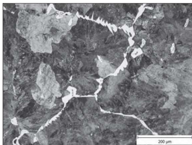
Obr. 2 Mikrostruktura plynule litého sochoru Fig. 2 Microstructure of continuously cast billet
