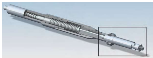
Obr. 1 Záchyt PRO-M (VVER 440/V) Fig. 1 Component of Capture Part PRO-M (VVER 440/V)
