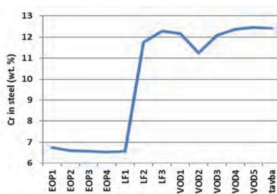
Fig. 16 The course of the content of Cr in steel during production in EAF and processing in LF and VOD of X2CrNiMo13-4 quality
